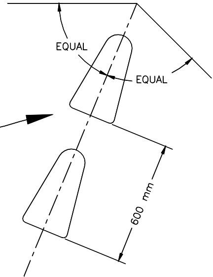
DETAIL-1 CORNER MOUNT
